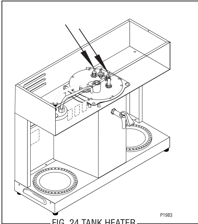
FIG. 24 TANK HEATER
